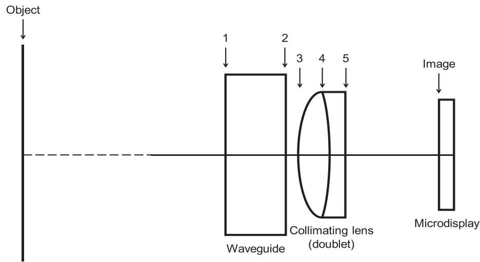
Fig. 15. Optical surfaces being engaged in the simulation. The optical path is arranged in the backward direction as the object—i.e. the virtual image of microdisplay—is located at the infinity. Waveguide is defined by surfaces 1 and 2, the diffractive properties of which are assigned as linear blazed gratings with opposite orders. Collimating lens is defined by surfaces 3, 4 and 5.
