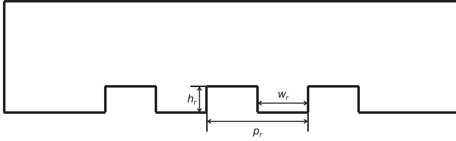
Fig. 7. Profile of relay grating, which is a rectangular or binary grating. h_r is the grating height, p_r the grating period, and w_r the grating width.
