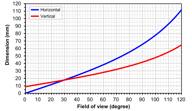
Fig. 14. As the horizontal/vertical FOV rises to 120^\circ , if the eye relief and exit pupil are unchanged, the required horizontal and vertical dimensions of out-coupling grating are 112 and 65 mm, respectively.
