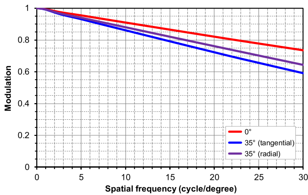
Fig. 16. MTFs calculated as a function of the spatial frequency in cycle/degree for the fields of 0° (central) and 35° (tangential and radial). At 30 cycle/degree, MTFs of all fields are above 0.591.
