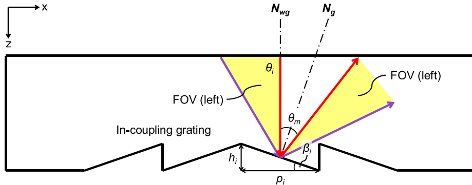
Fig. 6. Profile of in-coupling grating, which is composed of two blazed gratings with opposite directions. h_i is the grating height, p_i the grating period, \beta_i the slant angle, \theta_i the incident angle, \theta_m the diffraction angle of m th order, N_{wg} the waveguide normal, and N_g the grating normal.
