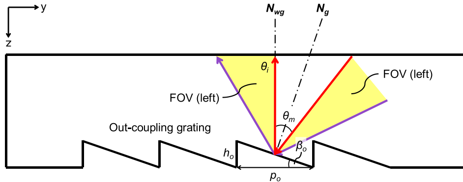
Fig. 9. Profile of out-coupling grating, which can be deemed as the conjugate of in-coupling grating for it would counteract the in-coupling grating and reverse the light back to its original state.
