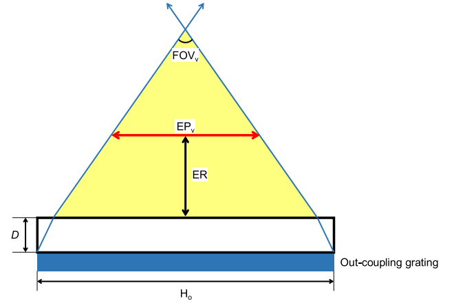
Fig. 13. Illustration of vertical exit pupil. For H_o = 20 mm, ER = 15 mm, and FOV_v = 38^\circ , EP_v = 9 mm.
