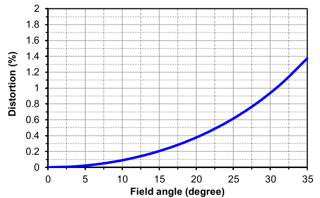
Fig. 17. Distortion calculated with respect to the field angle. It can be seen that the distortion up to the field of 35° is 1.38%.
